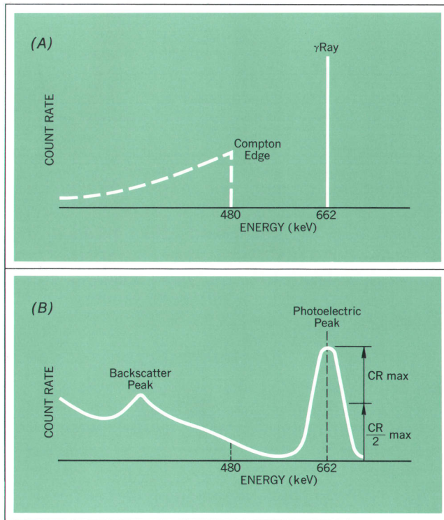
Fig. 3. Gamma spectra of Cs^{137} gamma radiation (A) Ideal, (B) Typical in practice.
